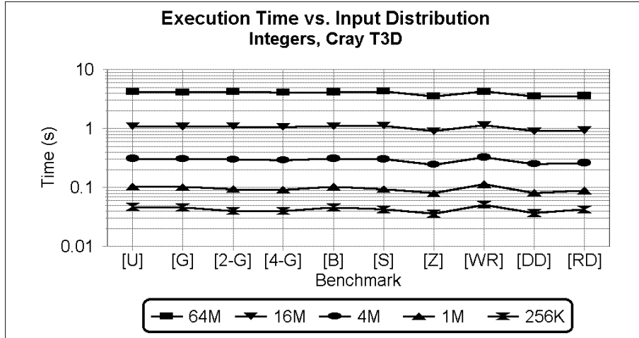
Fig. 3. Total execution time (in seconds) required to sort a variety of integer benchmarks on a 64-node Cray T3D.
