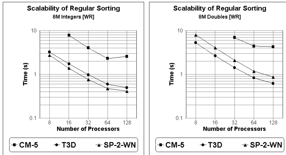
Fig. 7. Scalability of sorting integers and doubles with respect to machine size.
