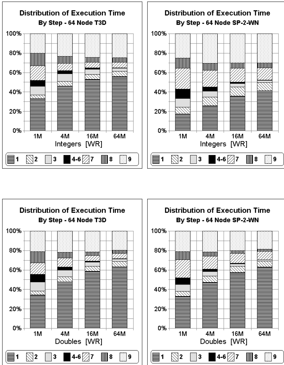
Fig. 9. Distribution of execution time amongst the nine steps of regular sample sort. Times are obtained for both a 64 node T3D and a 64 node SP-2-WN using both the integer and the double versions of the [WR] benchmark.
