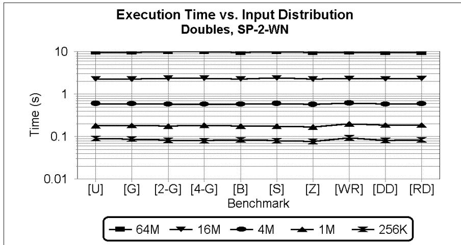
Fig. 6. Total execution time (in seconds) required to sort a variety of double benchmarks on a 64-node IBM SP-2-WN.
