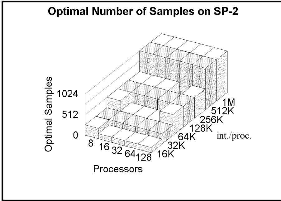
Fig. 2. Optimal number of samples s for sorting the [WR] integer benchmark on the IBM SP-2-WN, for a variety of processors and input sizes.
