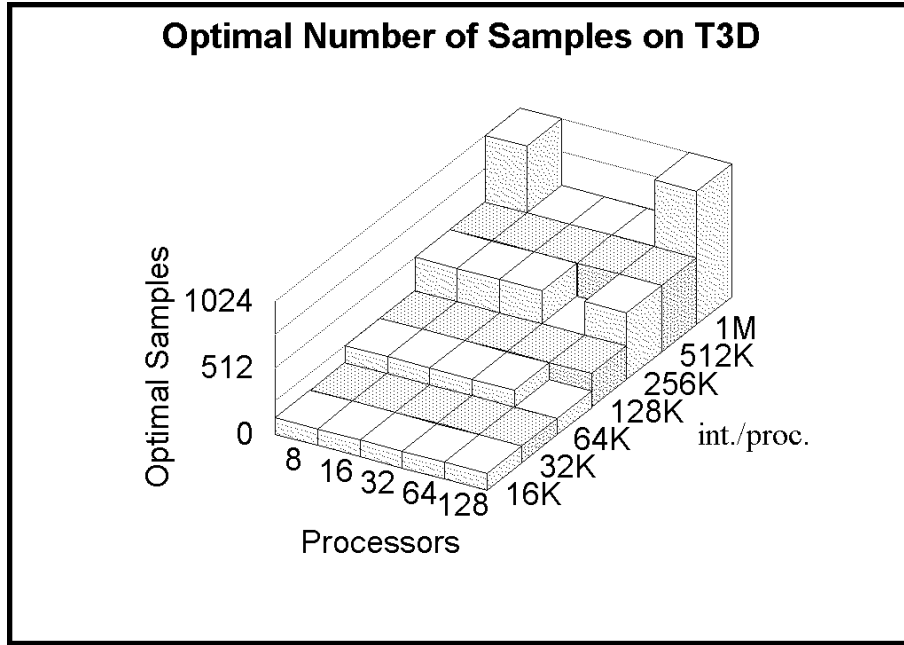
Fig. 1. Optimal number of samples s for sorting the [WR] integer benchmark on the Cray T3D, for a variety of processors and input sizes.
