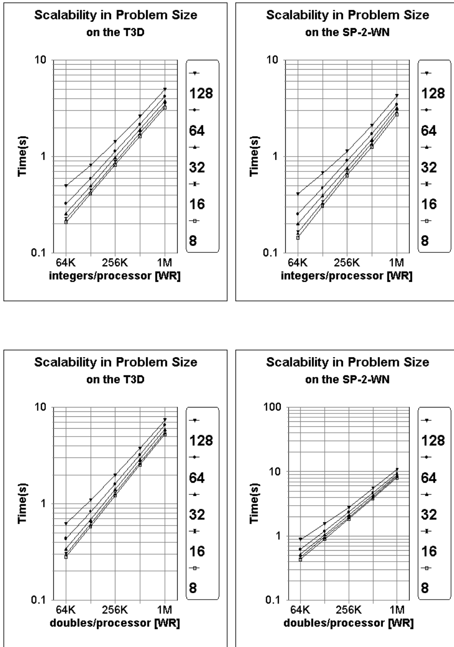
Fig. 8. Scalability of sorting integers with respect to the number of keys per processor ( \frac{n}{p} ), for differing numbers of processors.
