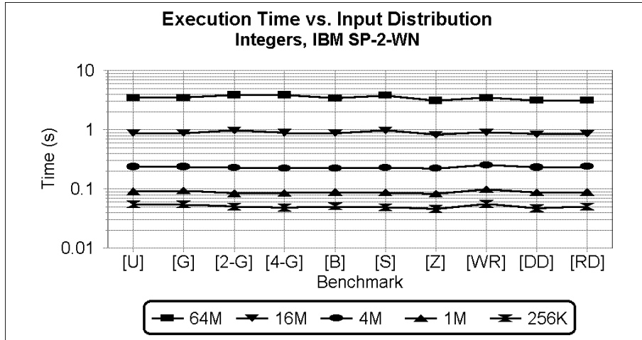
Fig. 4. Total execution time (in seconds) required to sort a variety of integer benchmarks on a 64-node IBM SP-2-WN.
