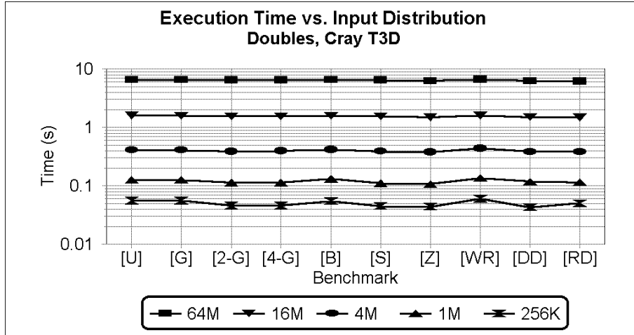
Fig. 5. Total execution time (in seconds) required to sort a variety of double benchmarks on a 64-node Cray T3D.
